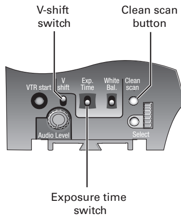
Figure 5-9. Exposure time controls
