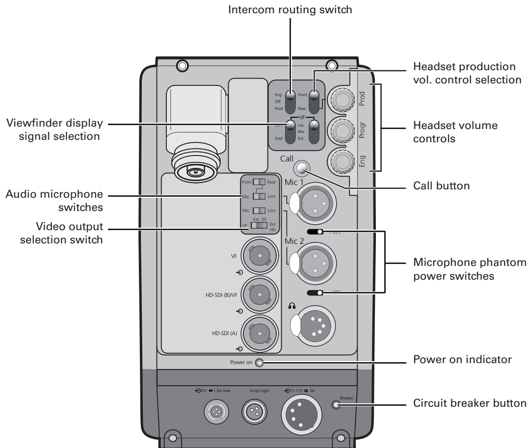
Figure 5-1. Rear controls
