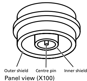
Figure 7-6. Triax connector
