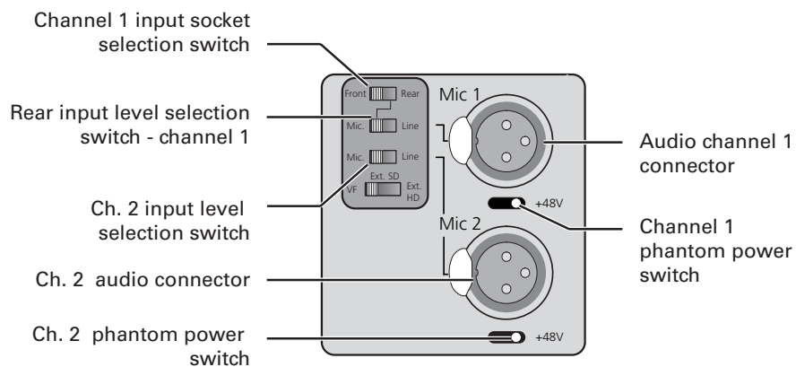
Figure 5-12. Audio channel switches
