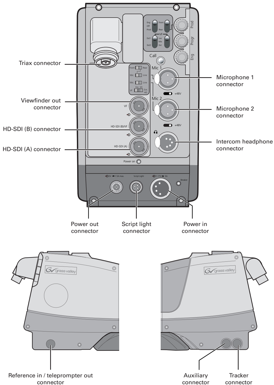
Figure 4-5. TriaxHD adapter connector location
